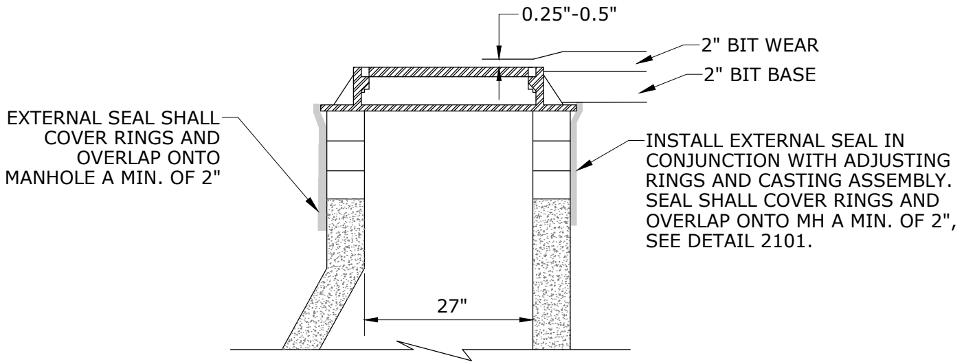
BIT. WEAR COURSE ADJ. DETAIL
