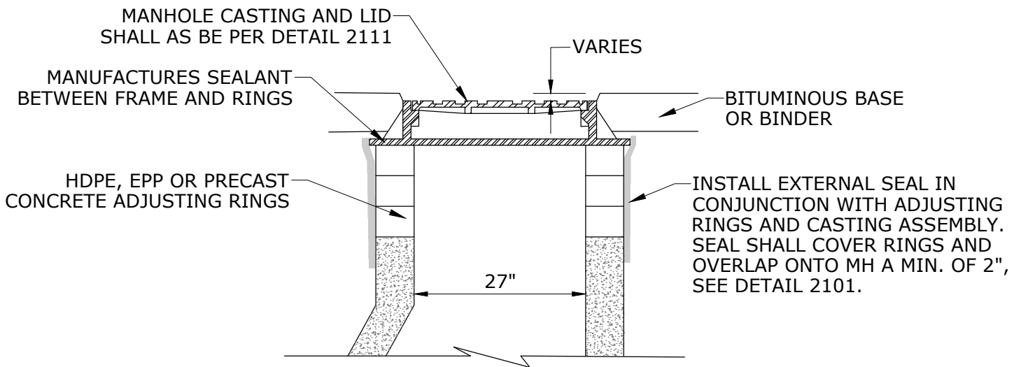
BIT. BASE OR BINDER COURSE ADJ. DETAIL
