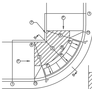
MODIFIED FAN (6) USED WHEN RIGHT-OF-WAY IS CONSTRAINED
