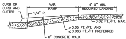
SECTION A-A PERPENDICULAR/TIERED/DIAGONAL
