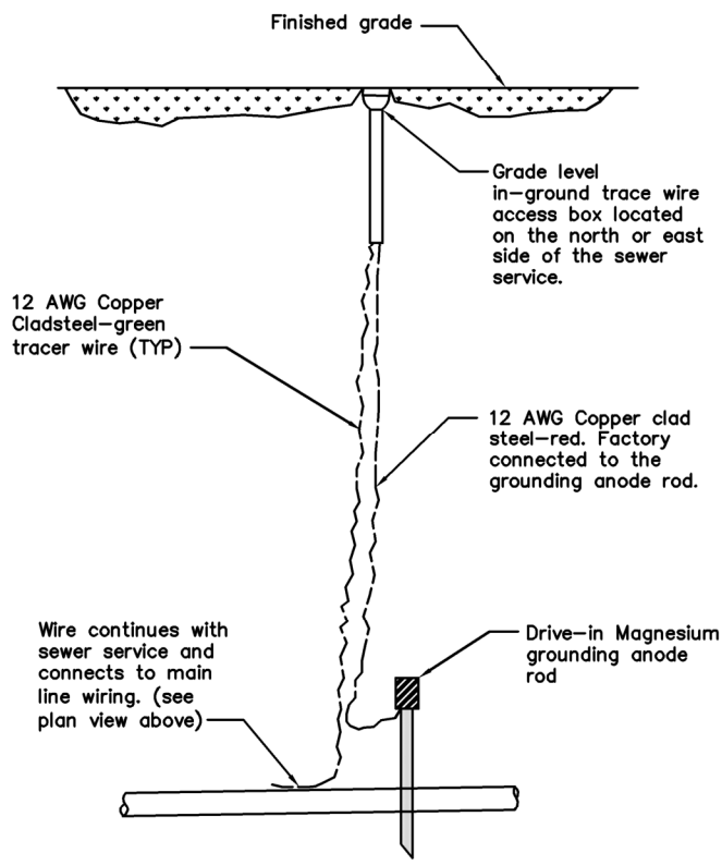
Sanitary Service-Section View Not to scale
